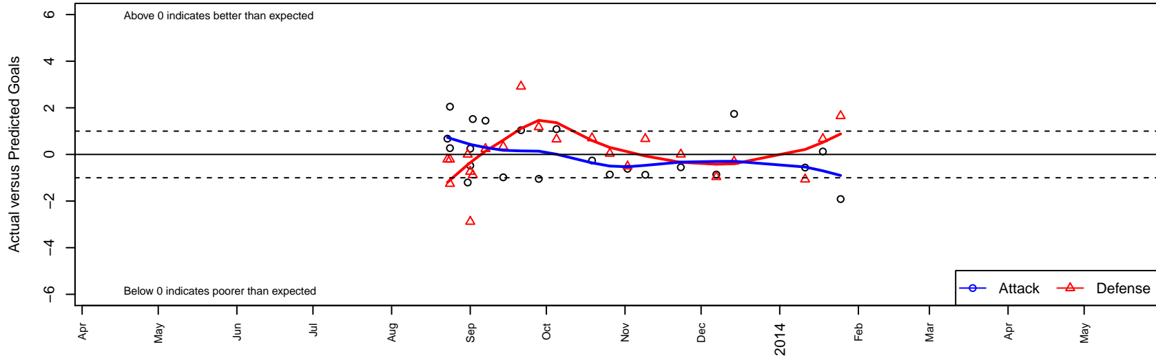
Mercer Island FC Tornado B99 Dots are actual minus expected GF (blue circles) and GA (red triangles). Blue line is smoothed change in attack strength. Red is smoothed change in defense strength.
